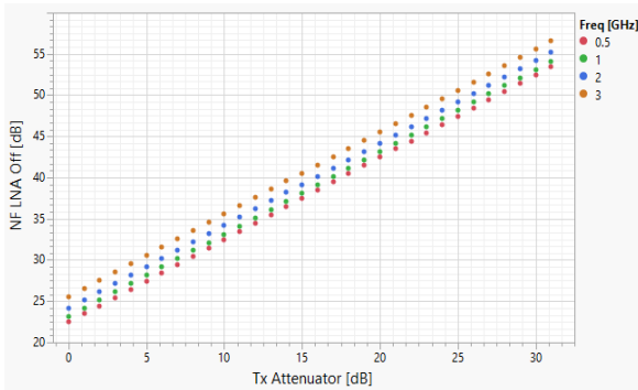
Noise Figure for 7 Freq. vs. Attenuator value, 2.5GHz RFoF - 'LNA Off'
