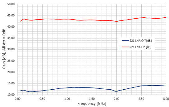
Gain vs. Freq. (S21), 2.5GHz RFoF 'LNA Off' (bottom), 'LNA On' (top)
