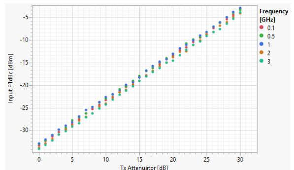
Input P1dBc at 7 frequencies, 2.5GHz RFoF - 'LNA On'
