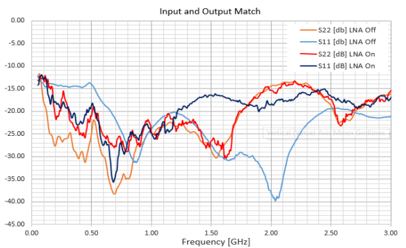
Input and Output Return Losses vs. Freq. (S11, S22) 2.5GHz RFoF 'LNA Off' and with 'LNA On'
