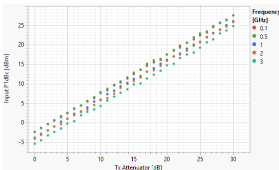
Input P1dBc at 7 frequencies, 2.5GHz RFoF - 'LNA Off'
