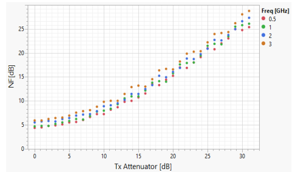
Noise Figure for 7 Freq. vs. Attenuator value, 2.5GHz RFoF - 'LNA ON'
