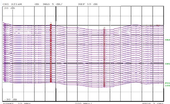
Gain vs. Tx Attenuation value: 0 to 31 dB in 1 dB step, 2.5GHz RFoF for 'LNA Off' (similar behavior for 'LNA On')
